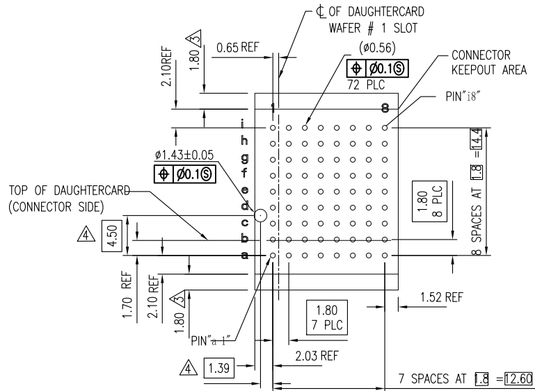
PC BOARD LAYOUT (CONNECTOR SIDE) (SEE SHEET 2 FOR RTM)
